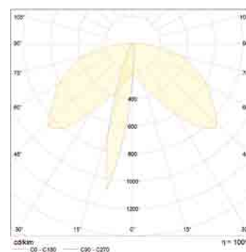
Wall-Washer WW
